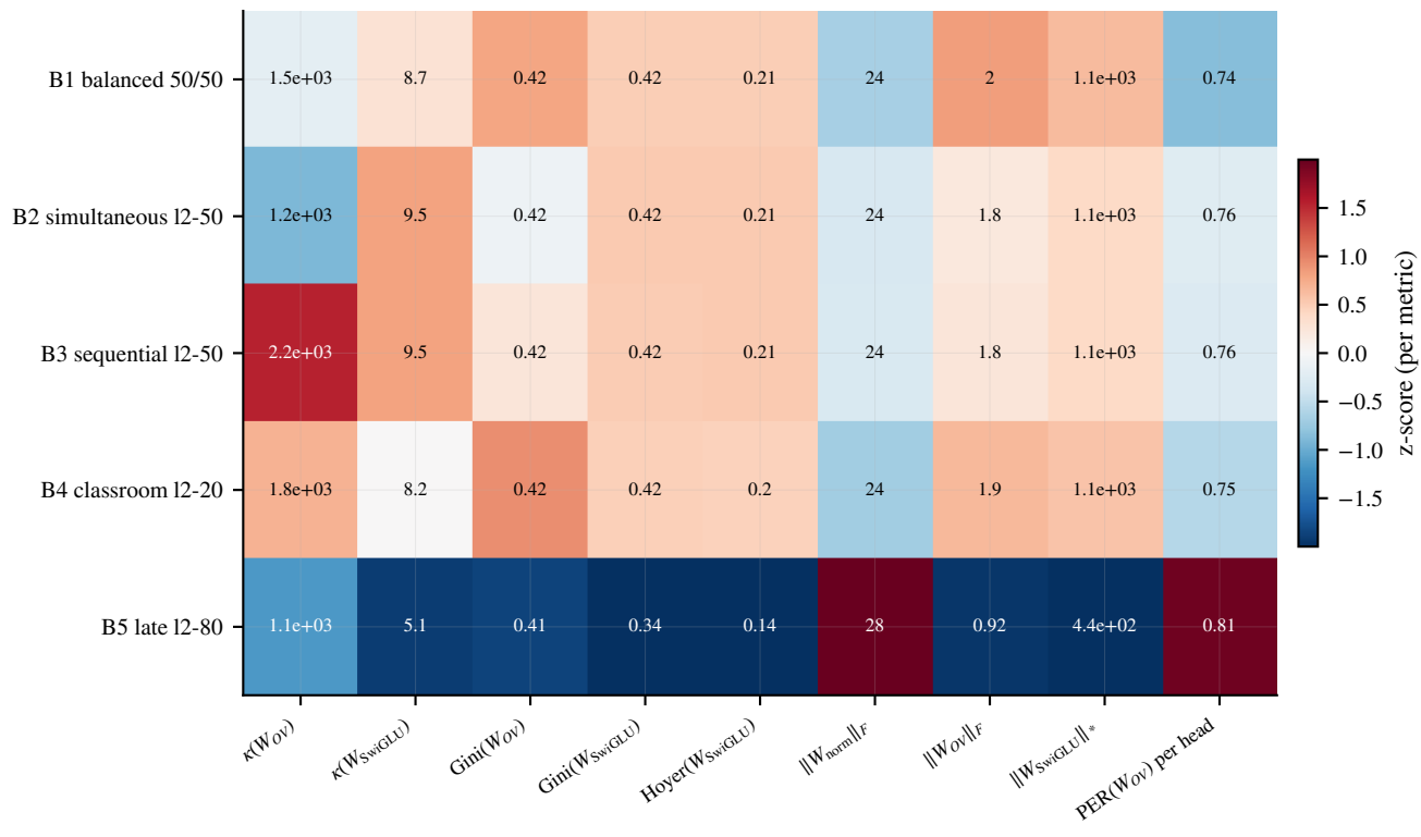
Q1b · Final-step interpretability across curriculum (nld→eng, FineWeb-100M)
